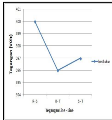
Gambar 10. Grafik Pengukuran tegangan line to line
