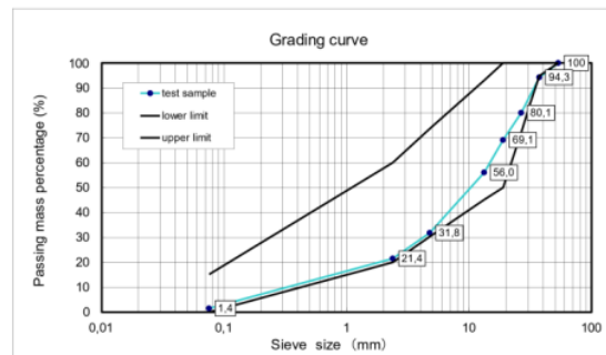
Gambar 4. Curva gradasi agregat base course eksisting
